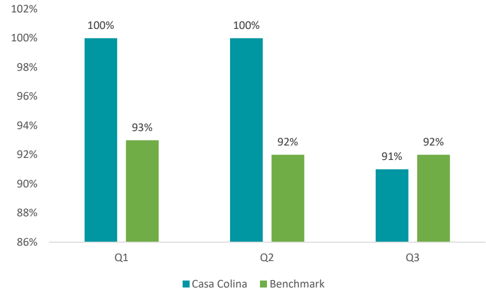
SCI: Remain in Community at 3 months
